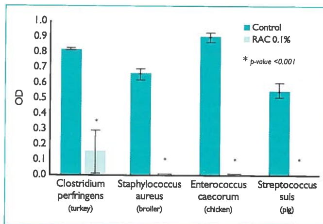
Fig. 1. The effect of RAC on the growth of pathogenic Gram positive bacteria in vitro (Alimetrics Ltd 2014). Clostridium perfringens was measured at five hours, Staphylococcus aureus and Enterococcus caecorum at eight hours, and Streptococcus suis at 10.5 hours.
